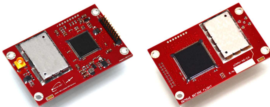
Fig. 8 Engineering Model of the piNAV-NG unit with Red Remove Before Flight finish - Top side (left), Bottom side (right).
