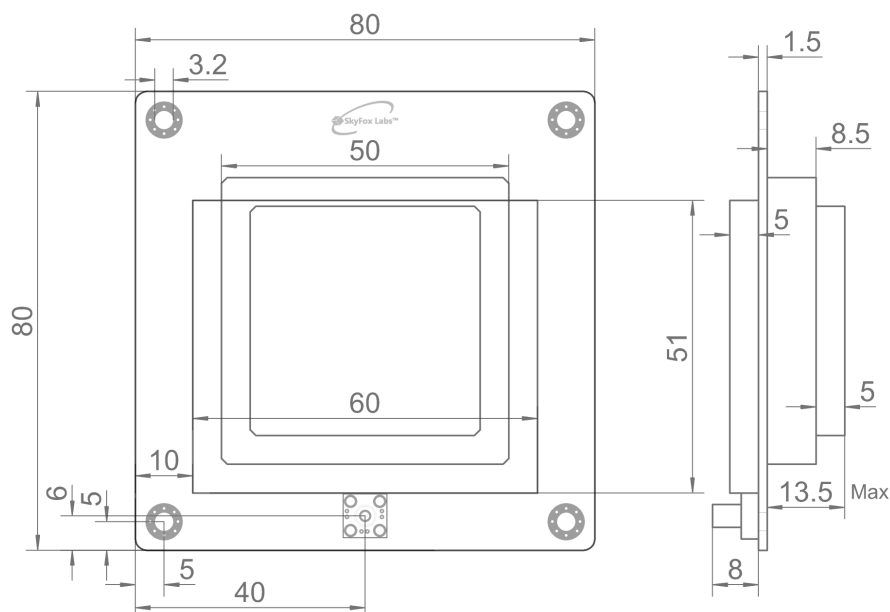
Fig. 2 piPATCH-AllBand-Midi Dimensions drawing in millimeters. Detailed STEP file available for download.
