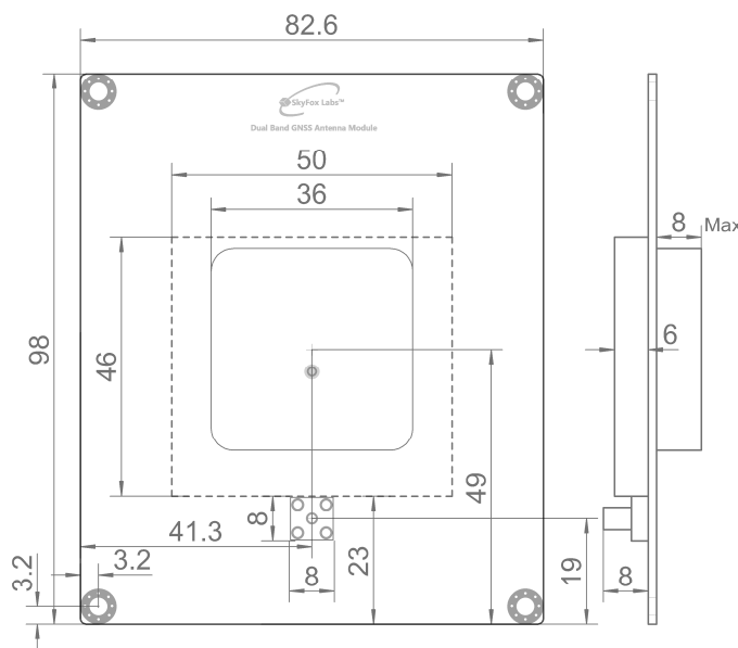
Fig. 2 piPATCH-DualBand Dimensions drawing in millimeters. Detailed STEP file available for download.
