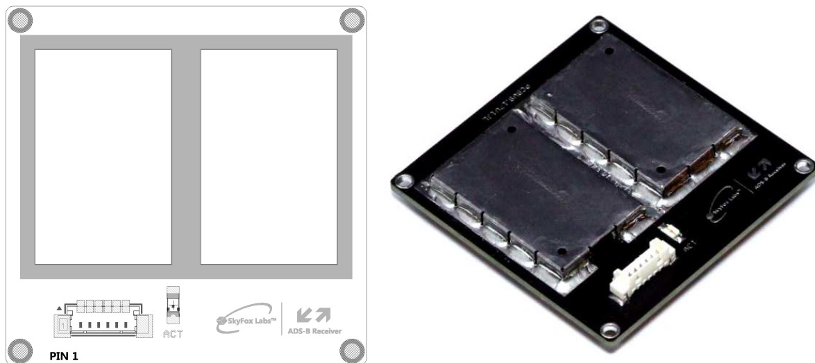
Fig. 2 The pqADS-B/FM Connector pinout and LED location . NOTE: The pqADS-B/FM is displayed from the BOTTOM side. The SMD mount connector type is MOLEX 53398-0671 with 1.25mm pitch. Detailed dimensions drawing is available online as STEP model.
