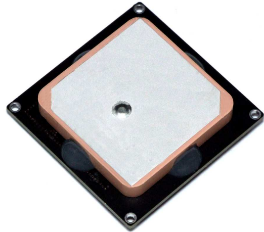
Fig. 1 Ultra Low Profile PocketQube ADS-B System, Flight Model.
