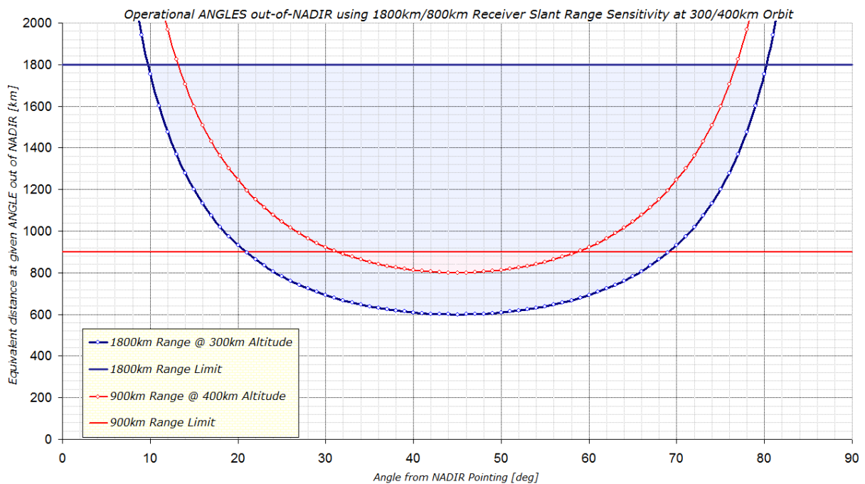
Fig. 5 Operational Angles out of NADIR for 300 and 400 km orbits.
