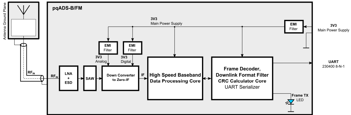
Fig. 3 The pqADS-B Receiver Block Diagram.
